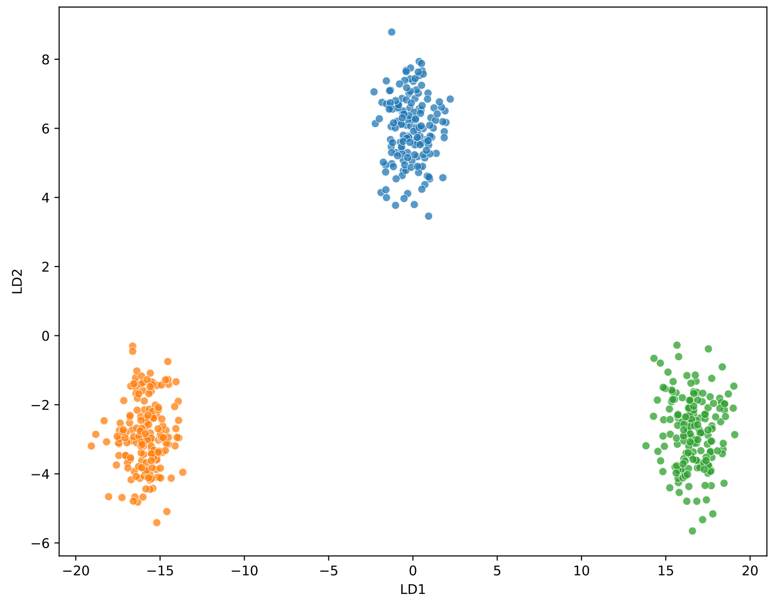
LDA
